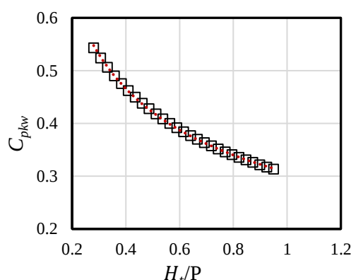
Fig. 6. Variations of discharge coefficient for piano key weir
