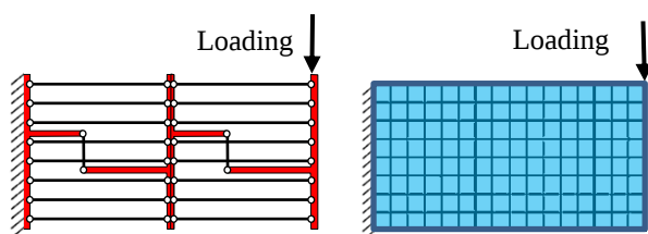
Fig. 10. Macroscopic modeling of the beam and its loading
