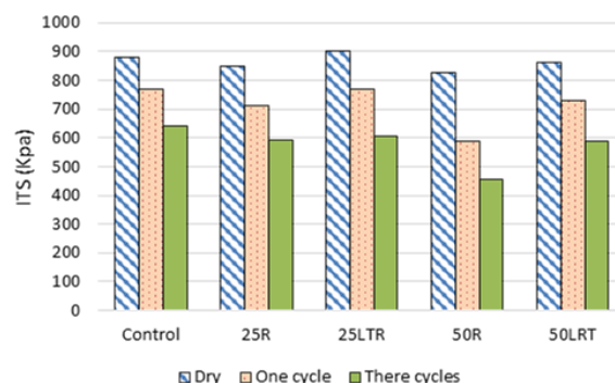
Fig. 3. Indirect tensile strength testing results of RCA content HMA
