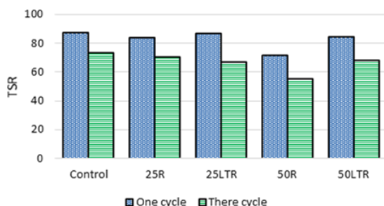
Fig. 4. Indirect Tensile Strength Ratio (TSR) of HMA mixes containing RCA
