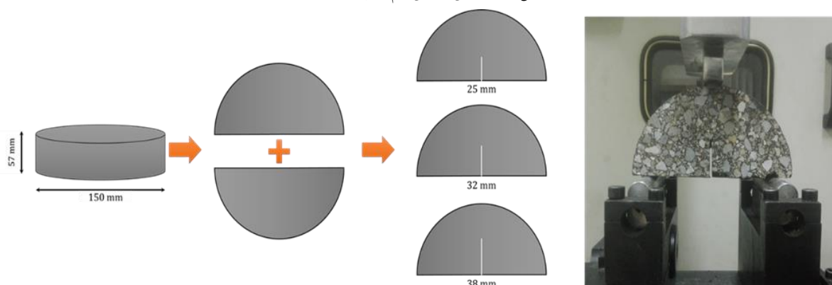
Fig. 2. Semi-circular bending (SCB) test
