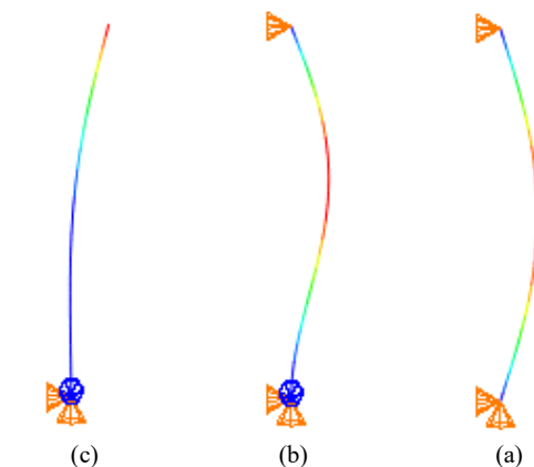
Fig. 15. The 1 st mode shape of the column with support conditions (a) pinned-pinned, (b) fixed-pinned and (c) fixed-free
