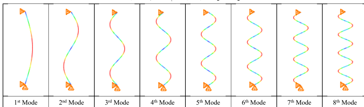
Fig. 2. Undamaged mode shapes of the column under the effect of axial load
