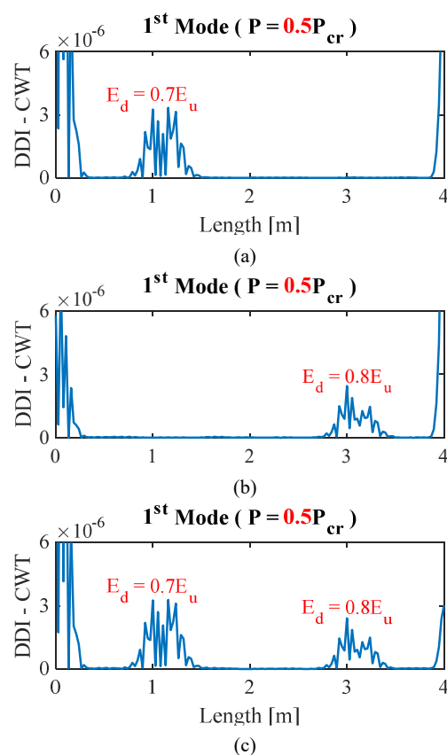
Fig. 4. DDI diagram of the 1 st mode resulting from continuous wavelet analysis of the db8 function for the (a) D1, (b) D2 and (c) D3 damage state
