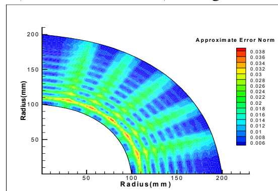
Fig. 24. Two-dimensional norm approximate error distribution in thick-walled cylinder.
