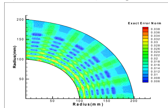
Fig. 23. Two-dimensional norm distribution of exact error in thick-walled cylinder.
