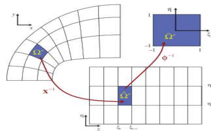
Fig. 2. Elements made by NURBS-shaped nodes and transfer mapping from (r, s) coordinate system to normal coordinate system [4].
