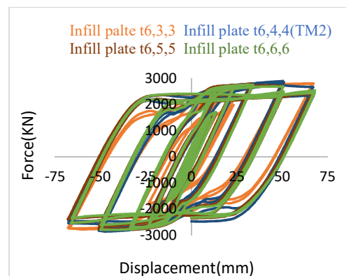
Fig. 25. Comparison of models with different thickness of steel shear wall infill plates equipped with ADAS t14 damper
