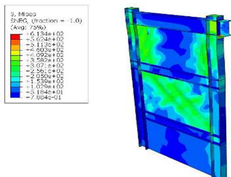
Fig. 3. Von Mises stress contour of TM2 specimen
