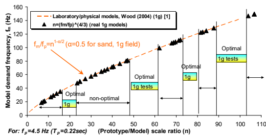
Fig. 16. Presentation of optimal and non-optimal frequency ranges for physical modeling in the 1g acceleration field to simulate the horizontal components of earthquake records.
