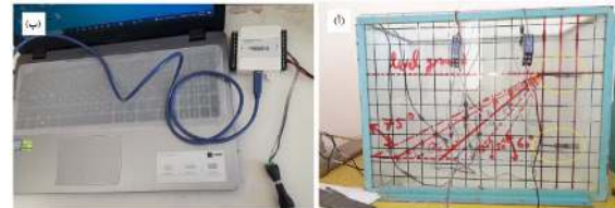
Fig. 10. (a) Deployment of acceleration sensors and electronic connection of signal conditioners; (b) Portable data card and connection of the whole set to the computer.
