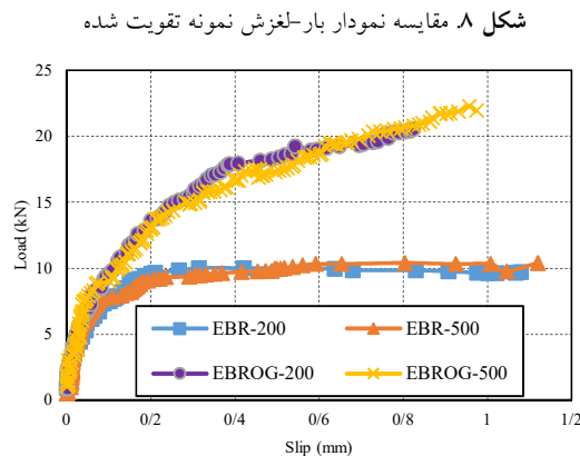
Fig. 8. Load-Slip curves
