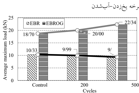
Fig. 5. Bar charts for strengthened specimens
