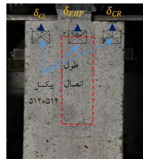
Fig. 6. Slip calculation
