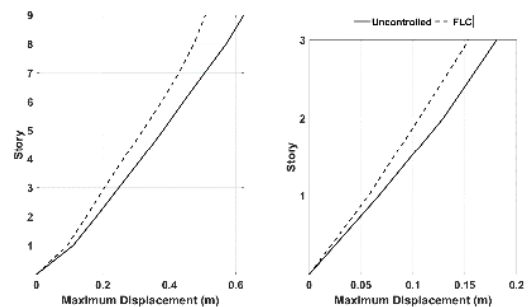
Fig. 18. Distribution of maximum floor displacement, Northridge, PGA=0.5g
