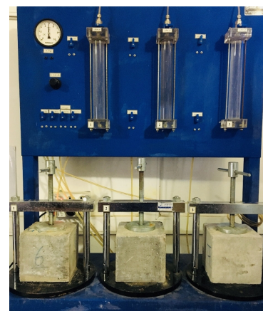
Fig. 5. Depth of penetration of water under pressure
