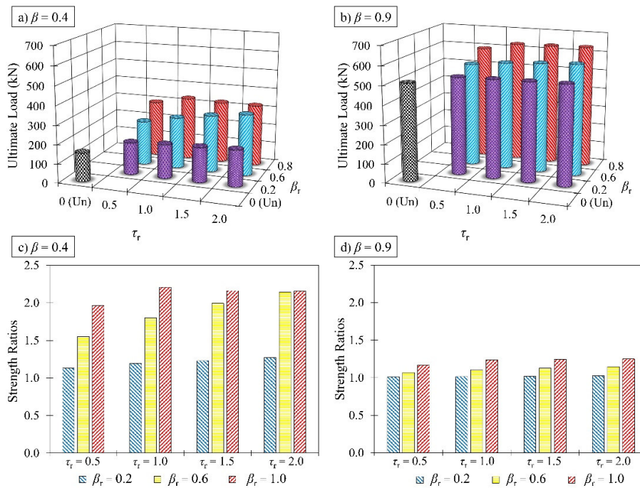
Fig. 7. The effect of the \beta on the ultimate strength values and ultimate strength ratios.
