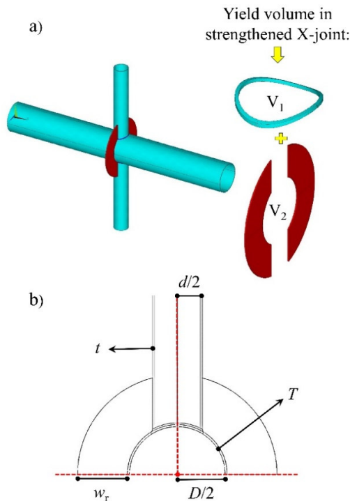
Fig. 13. a) Yield volume in stiffened and un stiffened joints, b) Calculation scheme to derive the relationship between the ratio of the ultimate strength of the stiffened joint to the ultimate strength of the corresponding unstiffened joint.
