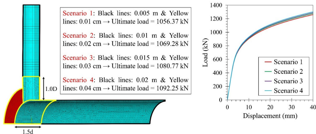
Fig. 4. Mesh sensitivity analysis.
