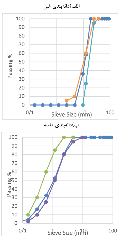
Fig. 1. The grain size distribution of the used aggregates
