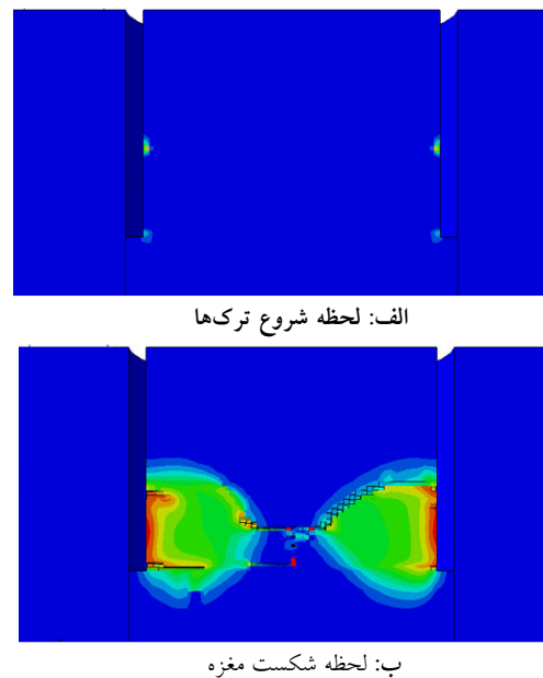
Fig. 12. The core failure in friction transfer test
