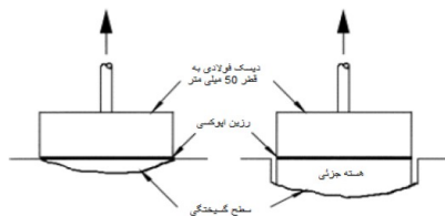
Fig. 1. View of the pull-off test
