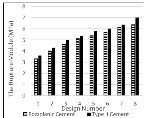
Fig. 20. The Rupture Module-Different Cements
