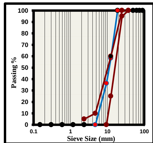
Fig. 1. Sieve Analysis of Coarse Aggregates.
