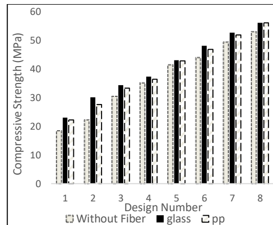
Fig. 14. Compressive Strength
