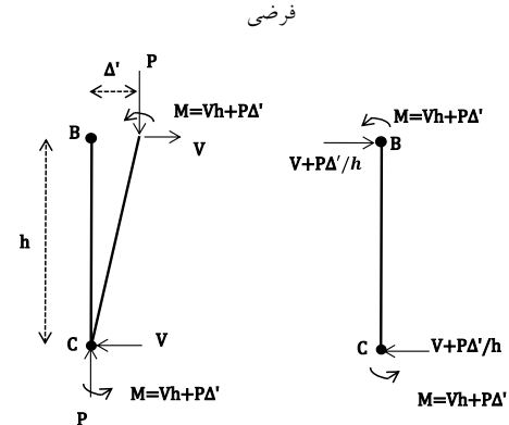
Fig. 1. Assumed shear in assume lateral load method (for consider of P-Δ effect)
