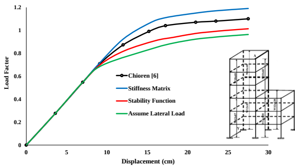
Fig. 5. Load-deflection curves of six story space frame
