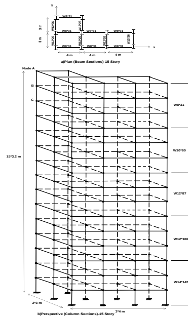
Fig. 10. Fifteen story space frame, a) beam section b) column section
