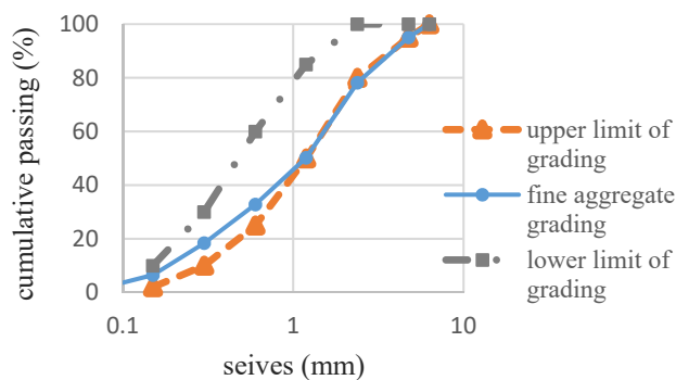
Fig. 4. Grading of fine aggregate according to ASTM C33 standard
