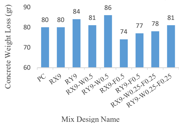
Fig. 11. Abrasion of control concrete and concretes containing 9% of rubber with wire and steel fibers
