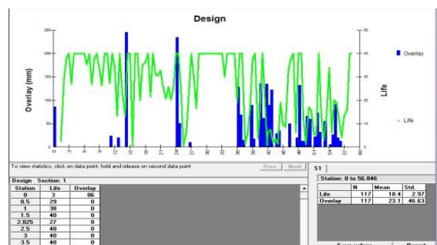
Fig. 2. Pavement thickness versus remaining life of a section of Ahvaz-Darkhoen Road
