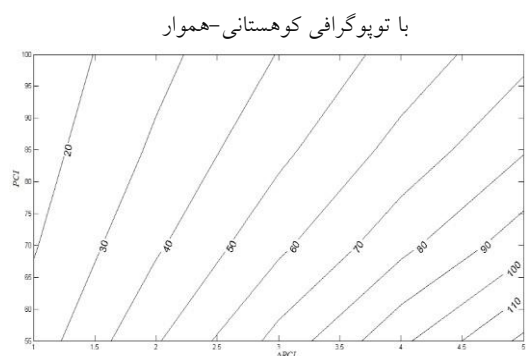
Fig 3. Remaining Service Life versus changes in PCI in roads in hilly topography
