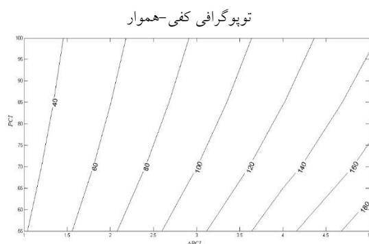
Fig. 4. Remaining life versus changes in PCI in roads in flat topography
