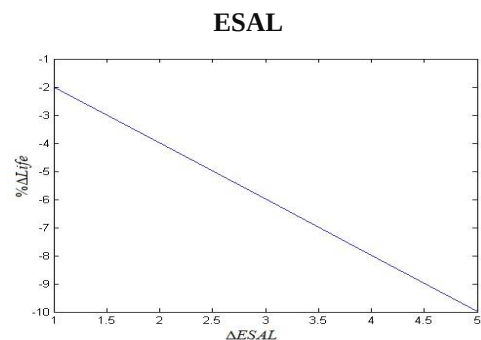
Fig. 5. Pavement remaining life versus changes in ESAL
