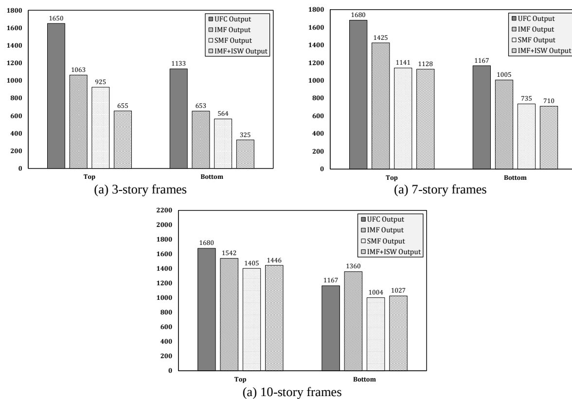
Fig. 7. Required rebar area in two ends of middle beams ( \text{mm}^2 )
