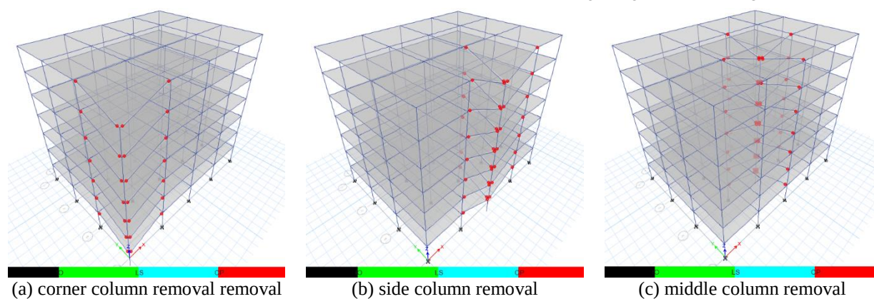
Fig. 2. Plastic hinges developed in 7-story intermediate moment frame under various column removal scenarios
