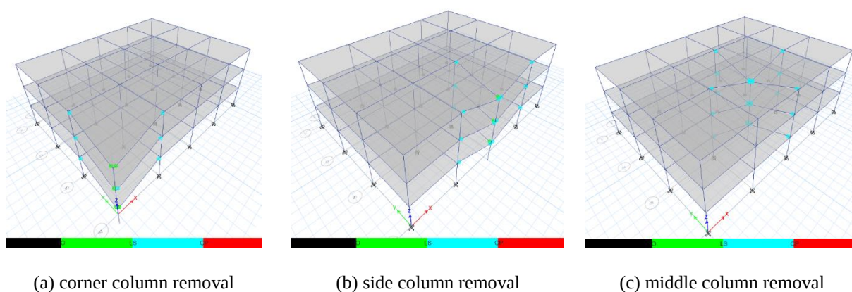
Fig. 9. Plastic hinges developed in 3-story frame designed using UFC provisions under various column removal scenarios
