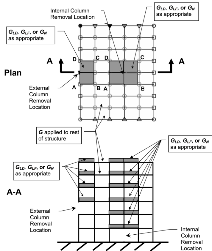
Fig. 3. Loads and Load Locations for Column Removal [14]
