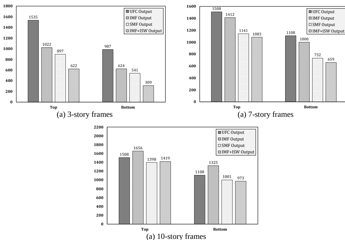
Fig. 6. Required rebar area in two ends of side beams ( \text{mm}^2 )
