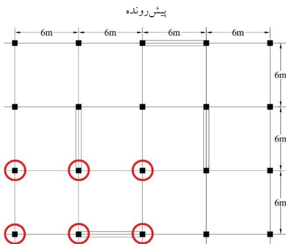
Fig. 4. Removed columns considered for progressive collapse design
