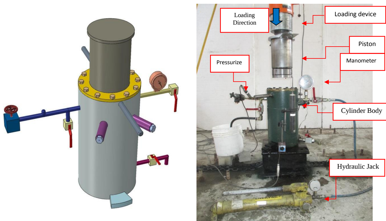
Fig. 4. Test set-up
