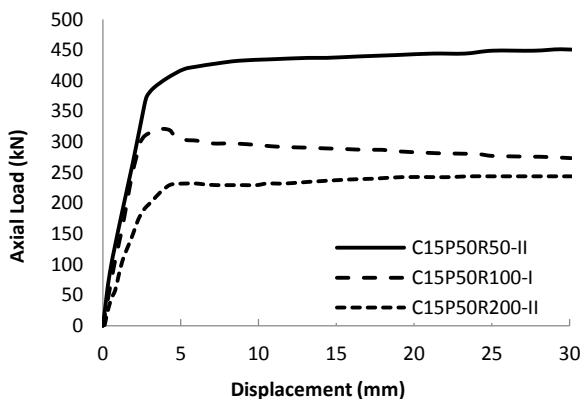
Fig.10. Load-axial deformation curves, 50 bar external pressure, 150 MPa concrete, D/t 50 , 100 , 200
