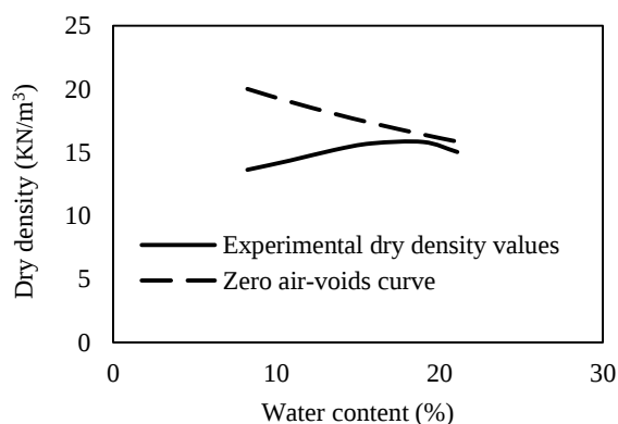
Fig. 1. Standard Proctor- compaction curve for soil
