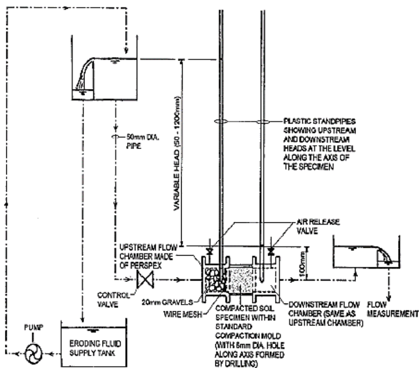
Fig. 3. Schematic diagram of Hole Erosion Test Assembly
