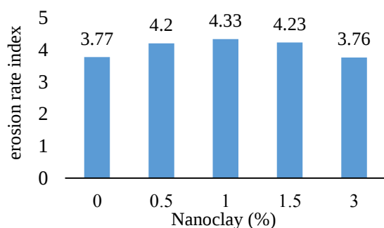
Fig. 6. Variation of erosion rate index versus amount of nanoclay for one-day curing period
