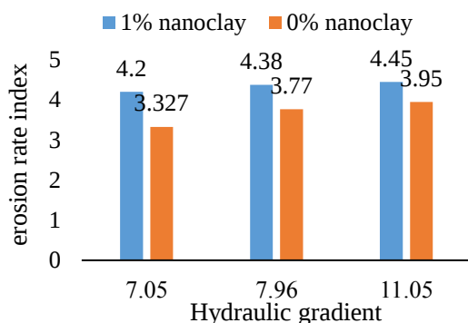
Fig. 9. Influence of hydraulic gradient on erosion rate index in the soil with 1% nanoclay and for one-day curing period.
