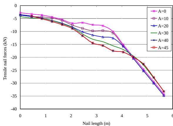
Fig. 11. Variation of tensile forces along the fifth row nails for different angles of the nails
