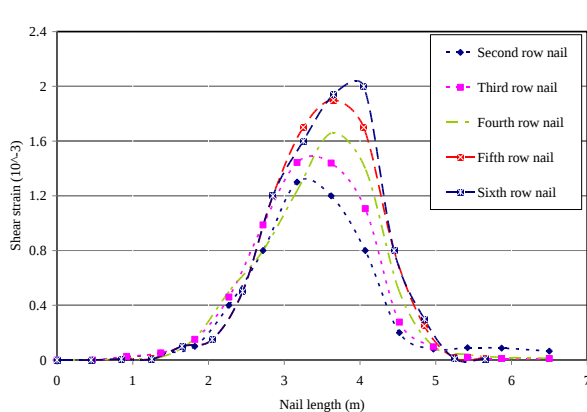
Fig. 13. Shear strain variations along the nailing angle of 30 degrees
