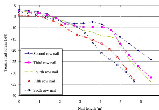
Fig. 15. The variation in the tensile strength of each six rows of nails for the angle of the nails with a horizon of 30 degrees
