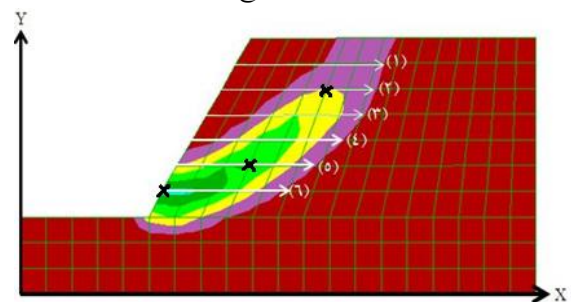
Fig. 7. Nailing model slope leading to Ilam-Salehabad road, and numbering them and the location of the nails through the wedge failure
