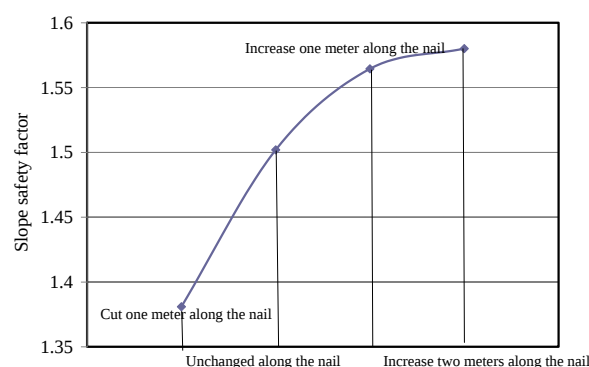
Fig. 20. Changes in the safety factor against changes in the length of the nails
