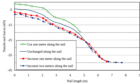
Fig. 18. The variation of the tensile force distribution along the fifth row nails for different lengths
