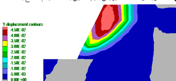
Fig. 4. Slope settlements contours of slope leading to the Ilam-Salehabad road
