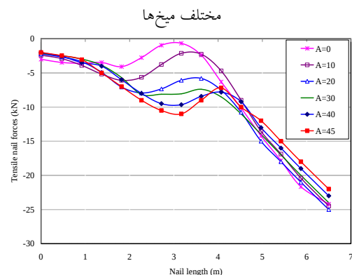
Fig. 8. Variation of tensile forces along the second row nails for different angles of the nails
