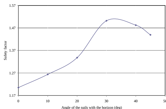
Fig. 14. Coefficient variations of safety factor against the angle of the nails with the horizon
