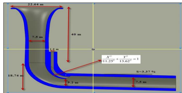
Fig. 3. Specifications of the Alborz morning glory spillway model
