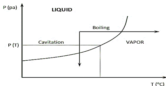
Fig. 2. Schematic diagram of cavitation occurrence
