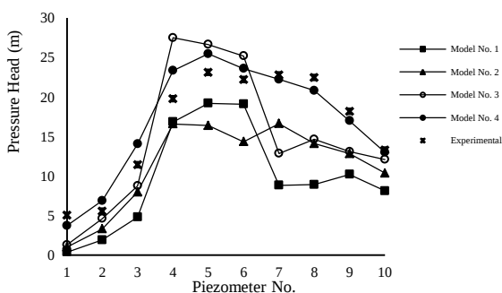
Fig. 6. Pressures taken at different points in the discharge 600 \text{ m}^3/\text{s} for different cell sizes
