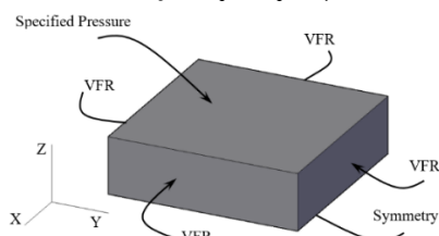
b. Boundary condition in Block 1
