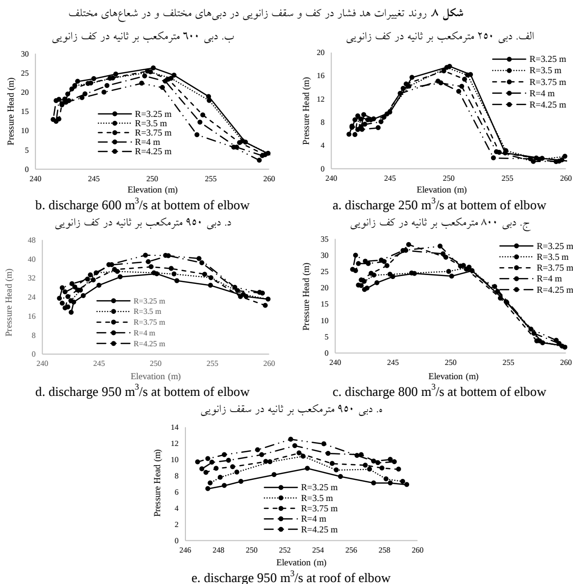
Fig. 8. Changes in the pressure in the elbow at different discharge and different radius of elbow
