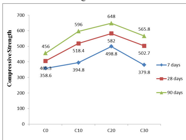
Fig. 4. Compressive strength of the replacement ratios (Kg/Cm²)
