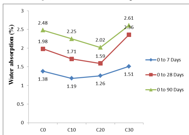
Fig. 7. Water absorption of the Replacement ratios
