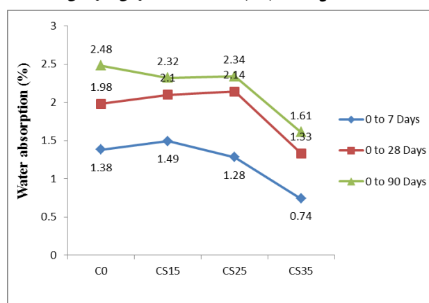
Fig. 8. Water absorption of the Replacement-additive ratios
