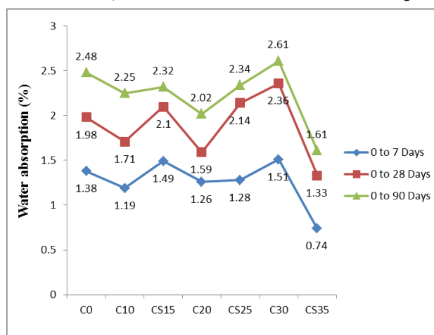
Fig. 9. Water absorption of samples containing various percentages of limestone powder
