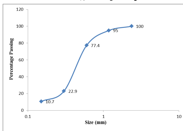
Fig. 1. Grading curve of the Limestone powder
