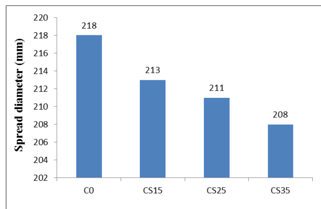
Fig. 11. Distribution of the flow table of the Replacement-additive ratios
