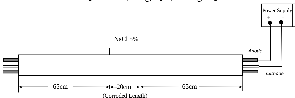
Fig. 2. Schematic representation of the accelerated corrosion test
