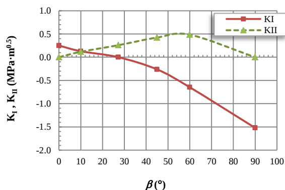
Fig. 8. Stress intensity factors in Modes I, II and mixed mode I-II for tested specimens ( a/R=0.3 , D=100\pm 1\text{mm} )
