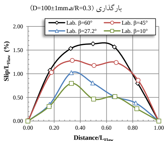
Fig. 13. Normalized slip distribution at closed flaw versus distance for various values of flaw inclination angle
