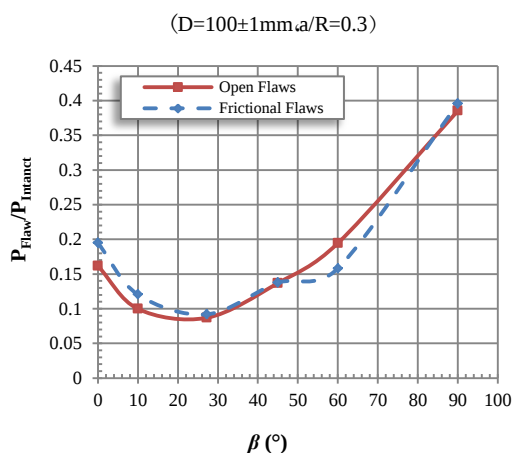
Fig. 11. Effect of flaw inclination angle on specimens normalized failure load (the failure load of specimens containing open and closed flaw divided to the failure load of intact specimen, a/R=0.3, D=100\pm 1\text{mm} )
