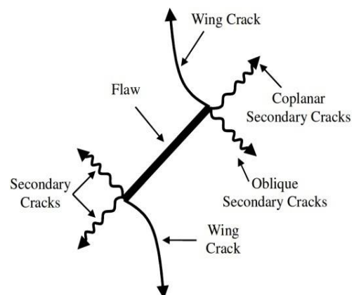
Fig. 2. Types of observed cracks initiated from a pre-existing flaw in rock materials under compression [32]
