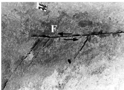
Fig. 1. Horsetail fractures at the end of a faulted joint (F), left-lateral shearing is shown by pair of arrows [11]
