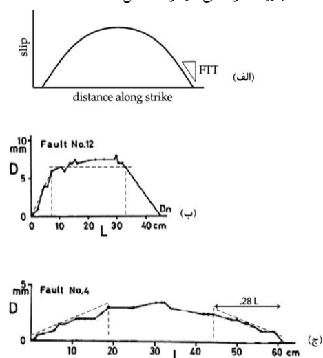
Fig. 14. (a) Expected displacement profile at a single fault without interaction and earthquake. (b) and (c) are examples of real faults, (D indicates slip) [40]
