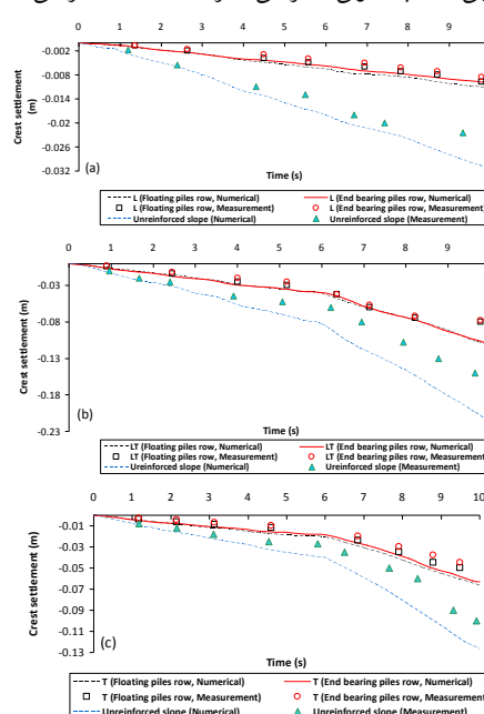
Fig. 11. Slope crest settlement in shaking table physical models for loading states: (a) L, (b) LT, (c) T.
