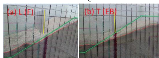
Fig. 10. Examples of slopes deformation after loading: (a) floating piles and L load, (b) end-bearing piles and T load.
