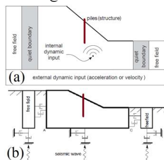
Fig. 6. Concepts of input motion and dynamic boundaries of the problem: (a) numerical model and dynamic boundaries; (b) waves dampers in free-field boundary.
