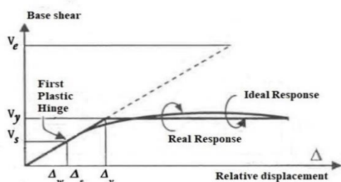
Fig. 4. Pushover curve [7]
