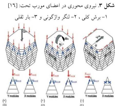
Fig. 3. Axial Forces in diagonal members: [16] 1- global Shear; 2- overturning moment; 3- gravity loads
