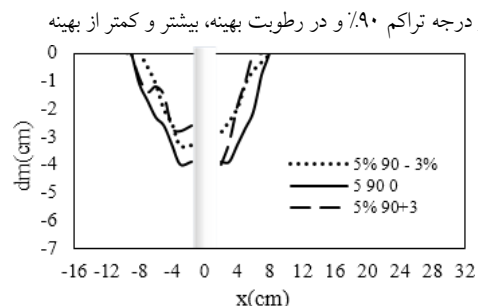
Fig. 9. Transverse scour profiles for sand + (5%) bentonite compacted with Dr = 90\% and Wc = w_{opt}, w_{opt} + 3\%, w_{opt} - 3\%
