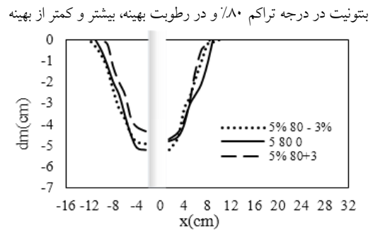
Fig. 8. Transverse scour profiles for sand + (5%) bentonite compacted with Dr = 80\% and Wc = w_{opt}, w_{opt} + 3\%, w_{opt} - 3\%
