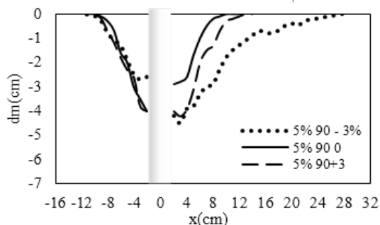
Fig. 7. Longitudinal scour profiles for sand + (5%) bentonite compacted with Dr = 90\% and Wc = w_{opt}, w_{opt} + 3\%, w_{opt} - 3\%
