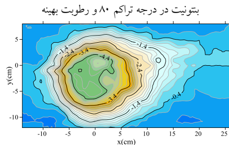
Fig. 10. Contour of scour hole for sand + (5%) bentonite, Dr=80\% , Wc= W_{opt}
