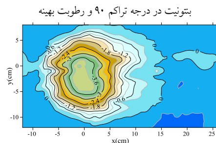
Fig. 11. Contour of scour hole for sand + (5%) bentonite, Dr=90\% , Wc= W_{opt}
