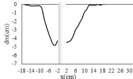
Fig. 17. Longitudinal scour profile for sand + (15%) kaolin compacted with Dr = 90\% and Wc = w_{opt}
