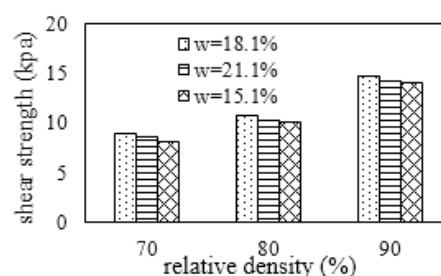
Fig. 13. Variation of shear strength versus relative density and water content for sand + (10%) bentonite
