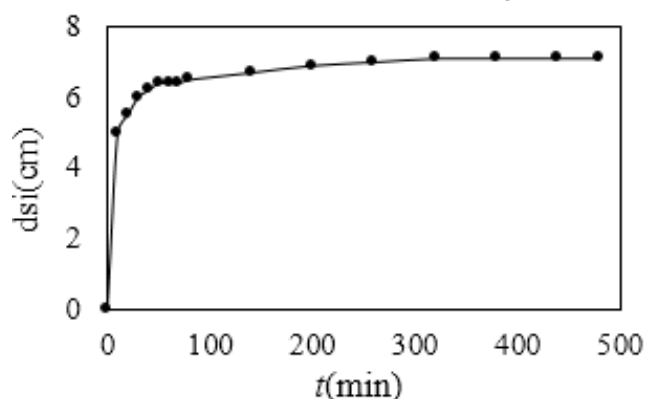
Fig. 1. Time development of scouring depth
