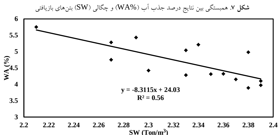
Fig. 7. The correlation between water absorption coefficient and specific weight
