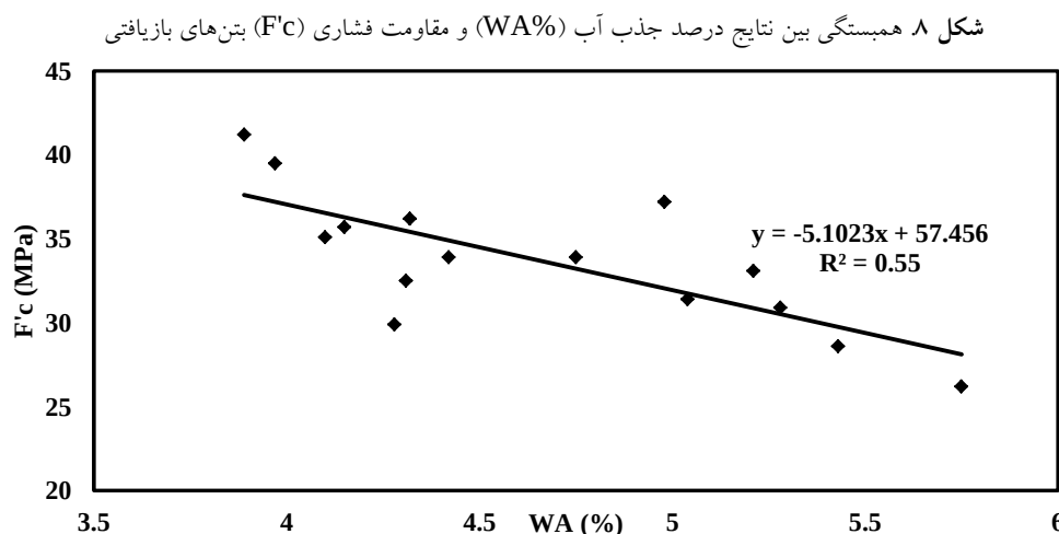
Fig. 8. The correlation between water absorption coefficient and 28-day compressive strength
