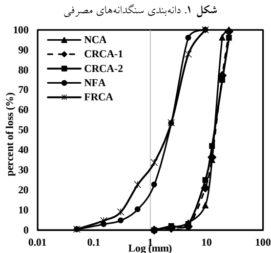
Fig. 1. Grading distribution of aggregates
