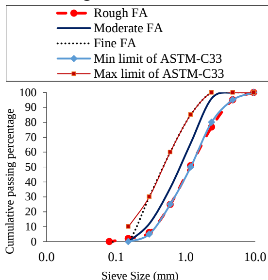
Fig. 2. Fine Aggregate grading curves
