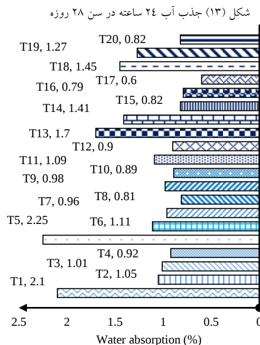
Fig. 13. Water absorption; 24 hours in age of 28 days
