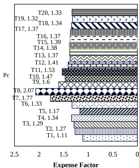
Fig. 4. Results of expense factor amount in all mixes
