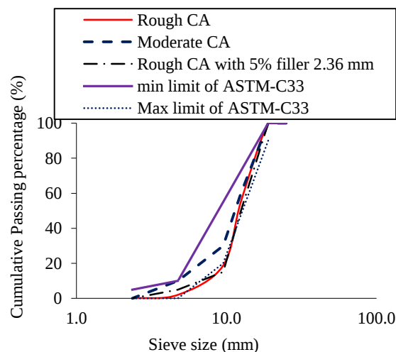
Fig. 1. Coarse aggregate grading curves
