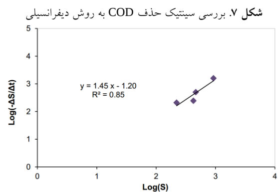
Fig. 7. kinetic of COD removal by Differential method
