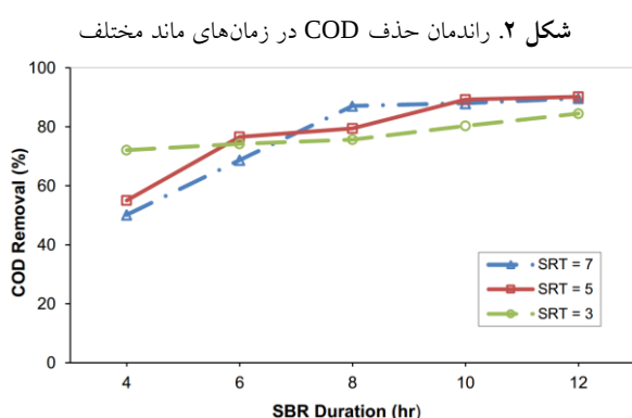
Fig. 2. COD removal at different retention time
