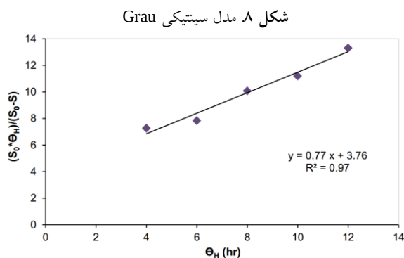
Fig. 8. Grau kinetic model
