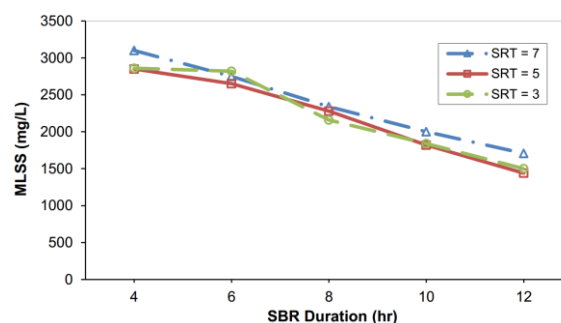
Fig. 4. variation of MLSS concentration at different retention time
