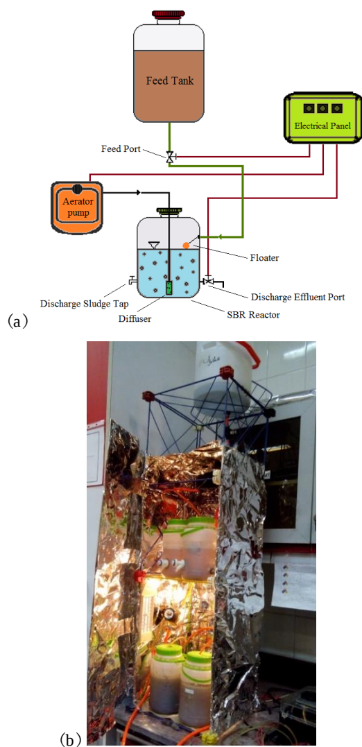
Fig. 1. schematic (a) and real shape (b) of SBR set-up
