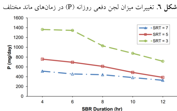
Fig. 6. variation of daily sludge production (P) at different retention time
