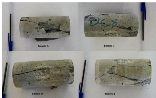
Fig. 9. Failure pattern of dry specimens with different porosity
