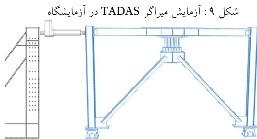
Figure 9: An illustration of the experimental setup
