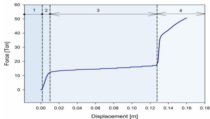
Figure 5: Force-Deformation relationship for the TADAS damper
