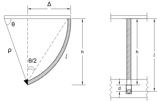
Figure 8: Schematic of the initial un-deformed, and deformed shape of a triangular plate in critical state
