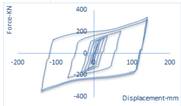
Figure 15: The hysteresis of the TADAS damper in ABAQUS
