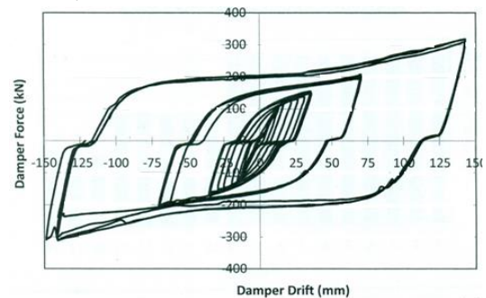
Figure 14: The hysteresis of the TADAS damper-The second test
