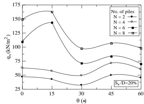
Figure (12): Variations of foundation pressure in terms of \theta .
