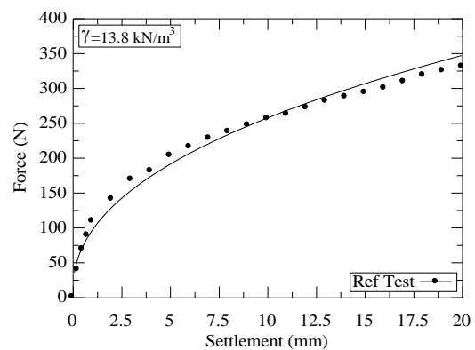
Figure (7): The load-settlement curve of Reference Test
