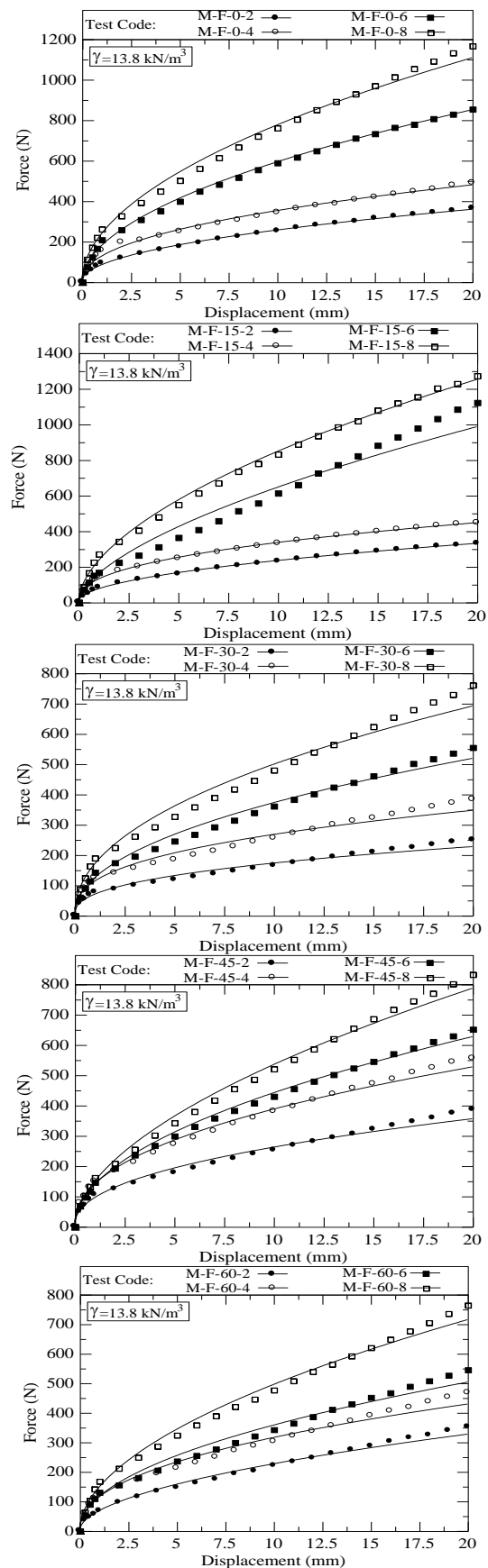
Figure (9): The load-settlement curve of M-F-Tests
