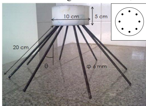
Figure (4-a): Set of micro piles and cap
