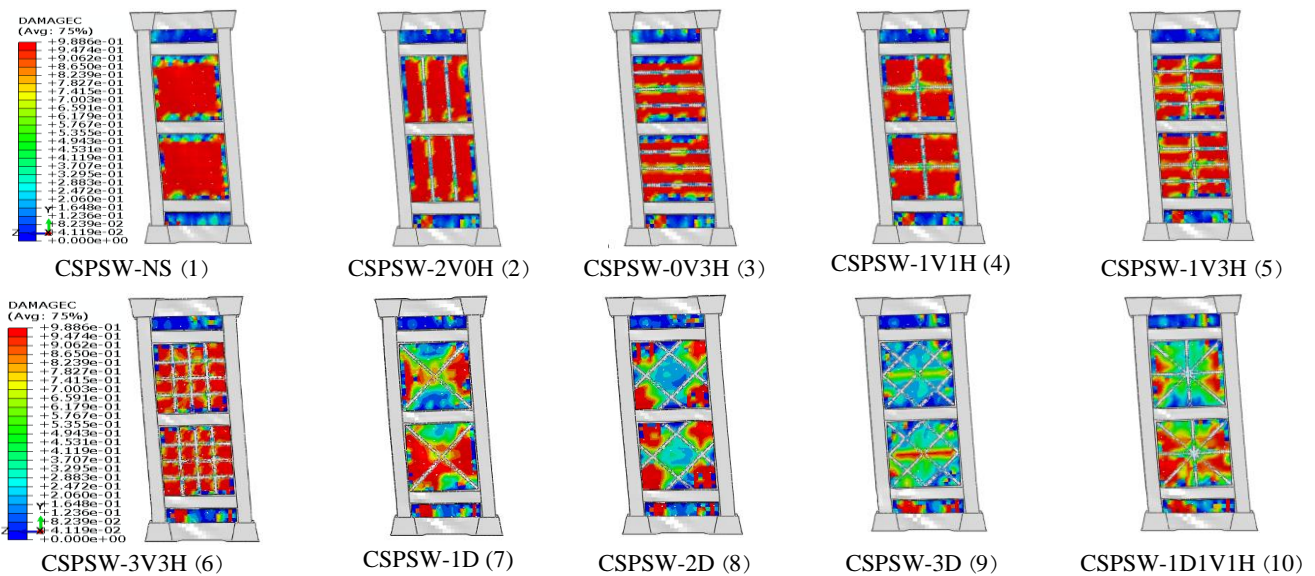
Fig. 15. Concrete compressive damage modes for parametric study from cyclic loading analyses
