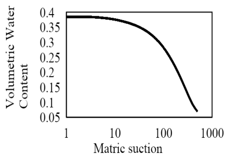
Fig. 1. swcc curve [12]
