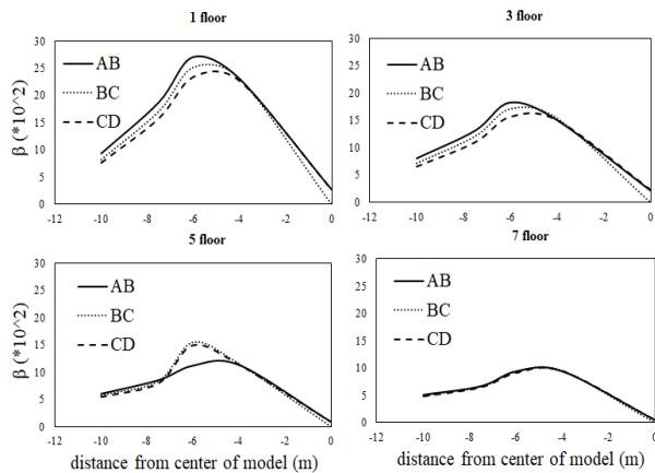
Fig. 22. The diagram of the angular distortion of the strip foundation, in different loading and for different positions of the pipe after one year
