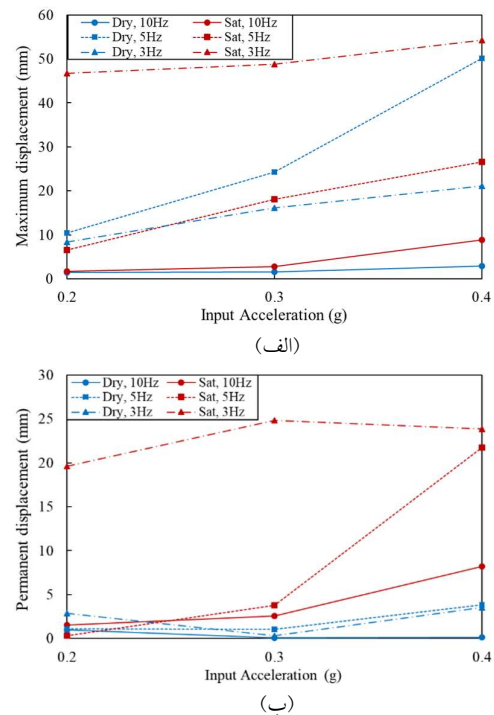
Fig. 10. Displacement-Input Acceleration diagrams of superstructure a) Maximum, b) permanent
