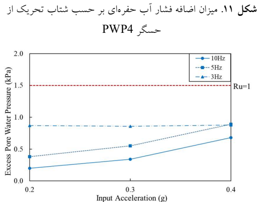
Fig. 11. Excess pore water pressure-input Acceleration diagrams of PWP4
