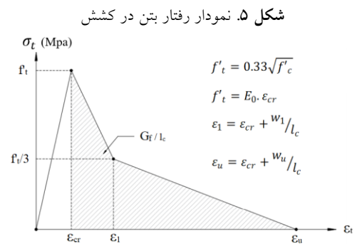
Fig. 5. Diagram of concrete behavior in tension
