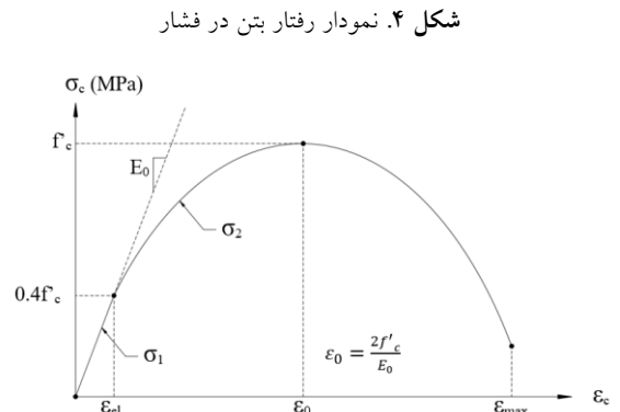
Fig. 4. Diagram of concrete behavior under pressure
