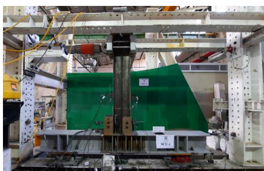
Fig. 8. Proposed self-centering connection test set up
