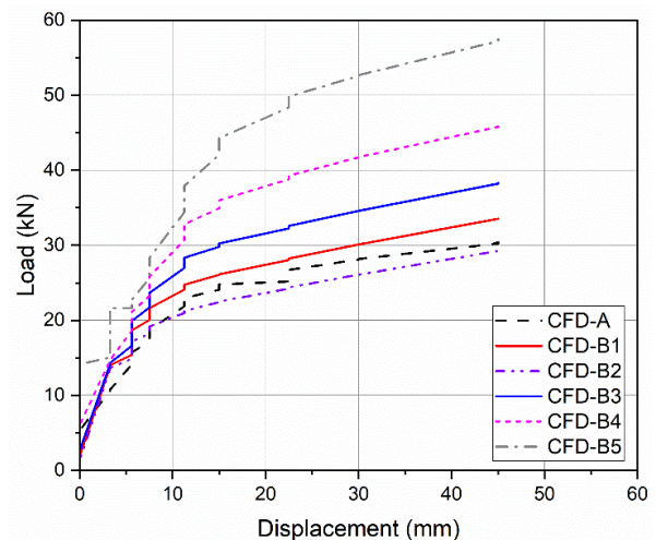
Fig. 19. Capacity curve of models
