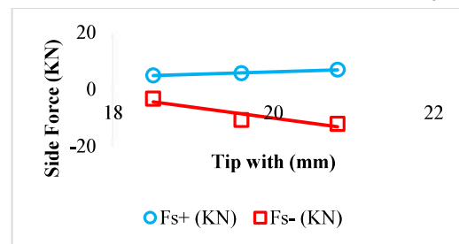
Fig. 10. Variation of side force with tip width
