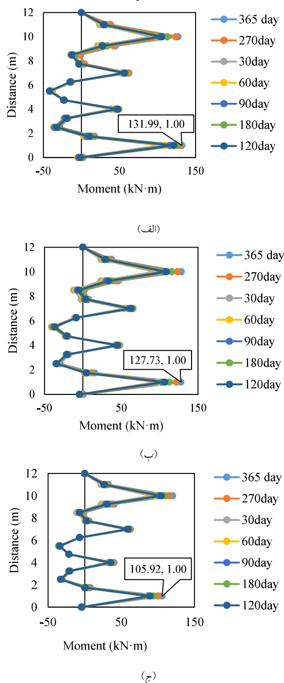
Fig. ۵ Diagram of bending moment-depth of the excavation wall for the stabilization excavation by anchoring method in the vicinity of the absorption well. a) 3 meters, b) 5 meters, c) 8 meters from Jadhargod
