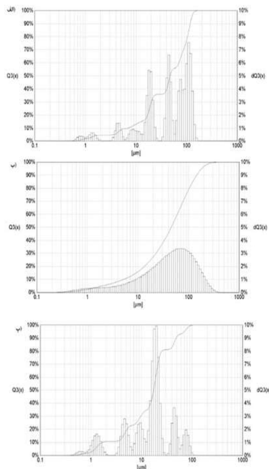
Fig 3- Particle size distribution of a) control reactor, b) reactor 1 and c) reactor 2.
