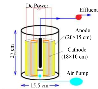
Fig 1- Pilot schematic electro membrane reactor
