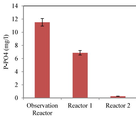
Fig 7- Phosphate Changes
