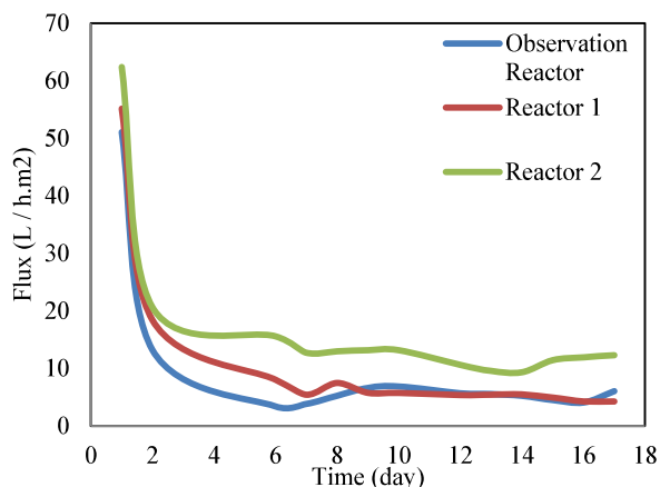
Fig. 8. Flux changes from the membrane
