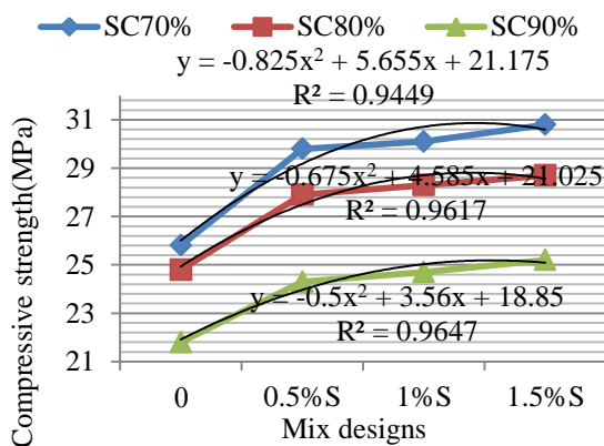
Fig. 4. The relationship between compressive strength and different percentages of steel fibers
