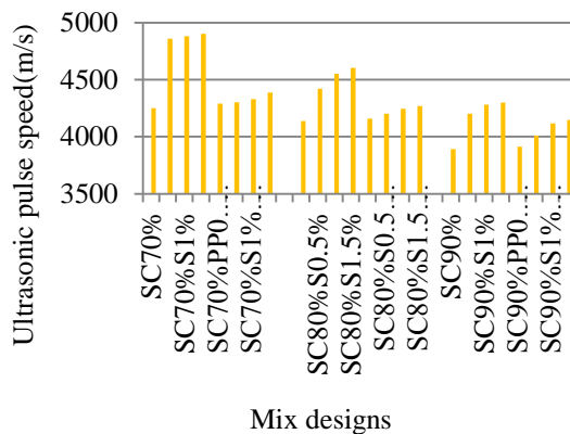
Fig.11. 28-day ultrasonic pulse speed of samples containing different percentages of steel and polypropylene fibers (m/s)
