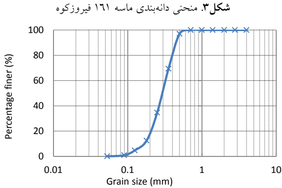
fig. 3. Grain size distribution curve of Firuzkuh sand (No.161)
