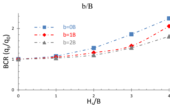
fig. 8. Variation in bearing capacity ratio in terms of H_s/B and b/B
