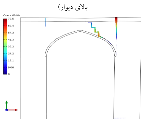
Fig. 17. The distribution pattern of cracks at the ultimate shear capacity for the wall with 0.15 MPa pre-compression gravity load intensity (average displacement of 49.5 mm at the top of the wall)
