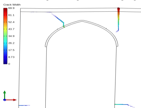
Fig. 8. The distribution pattern of cracks at the ultimate shear capacity of the wall without pre-compression gravity load (average displacement of 115.3 mm at the top of the wall)
