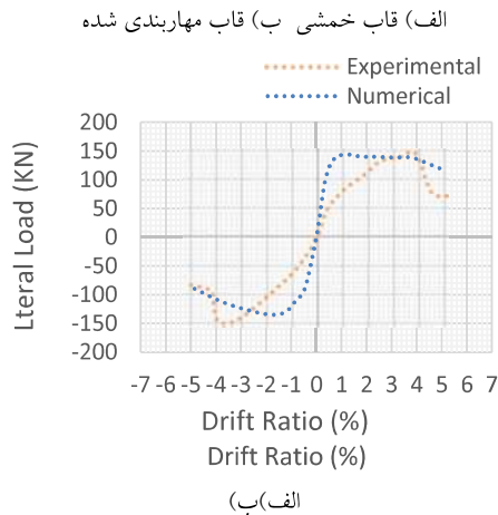
Fig. 11. Back bone curves a) moment frame b) barced frame
