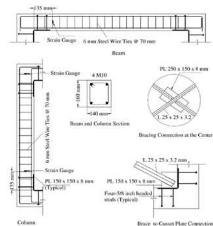
Fig. 4. Detailing of the braced RC frame [20]
