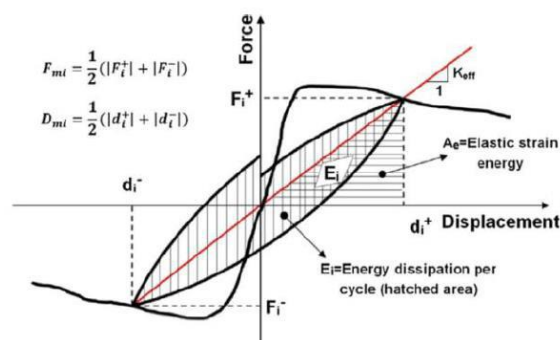
Fig. 17. stiffness calculation in each cycle [5]
