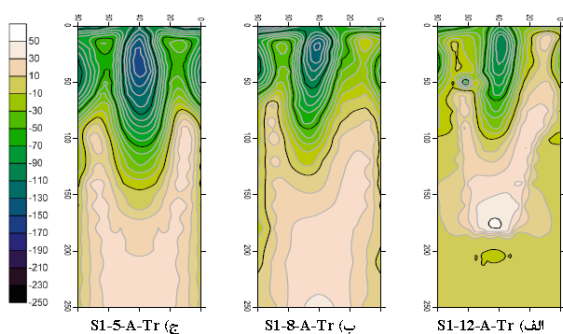
Fig. 4 Downstream topography for different Fr with stepped end sill
