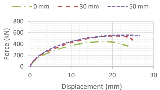
Fig. 17. Force-displacement diagram in different shotcrete thickness for beam No. 2
