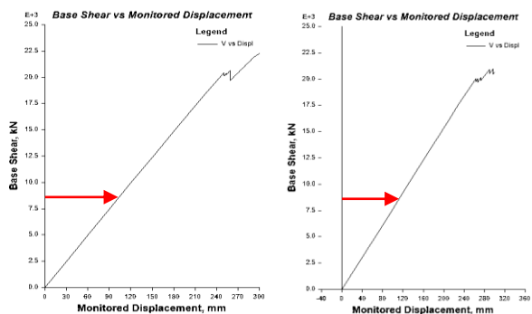
Fig. 7. Pushover curve for 15 story structure: push in the X direction (right) and push in the Y direction (left)
